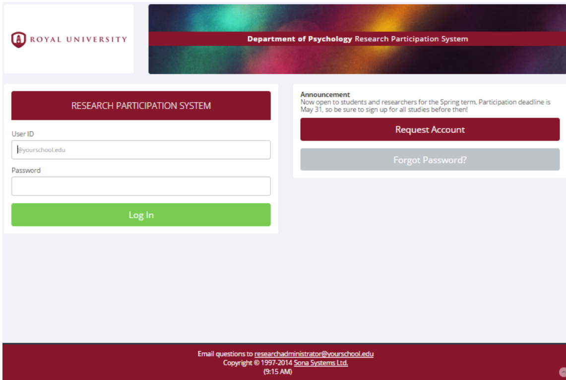
Figure 1 - Login Page
