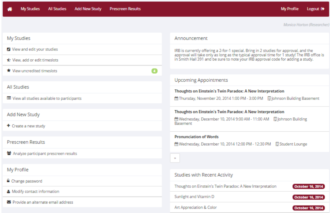
Figure 2 - Main Menu
